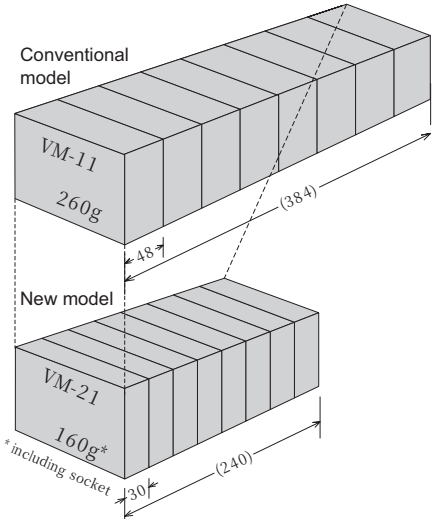
Example of 8 module mounting
