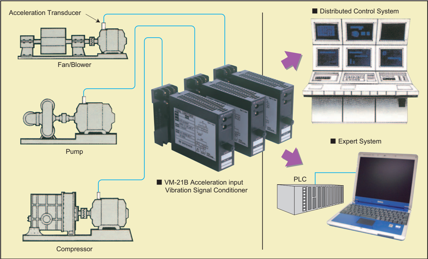
Typical Application
