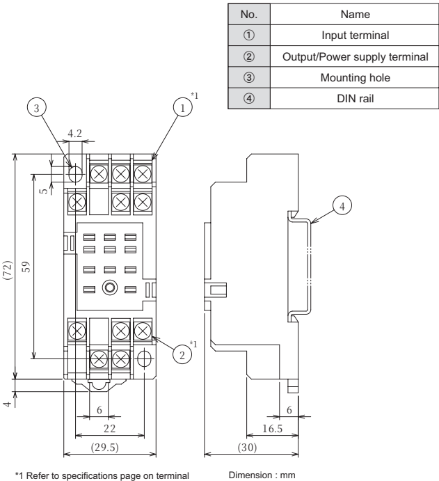
VM-21G Signal Conditioner Socket
